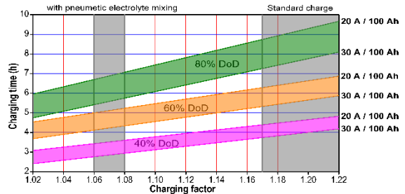
Charging times with IUla-characteristics in hours for PzS batteries at 30 °C
